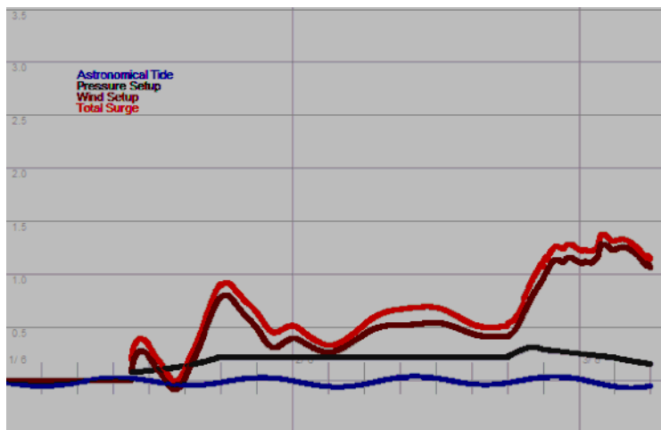
Figure 3. Storm surge generated by a category 1 hurricane (conditions stated under Results 2).
